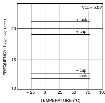
Fig. 18 Capture range / lock range vs. temperature
